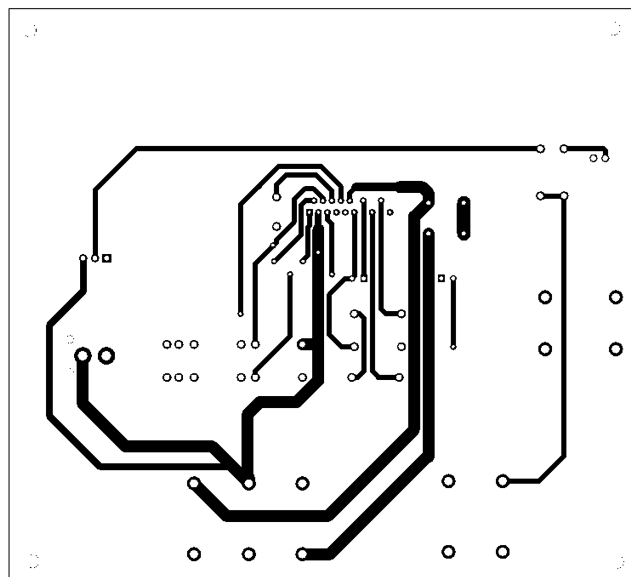
Figure 38. Bottom Layer
