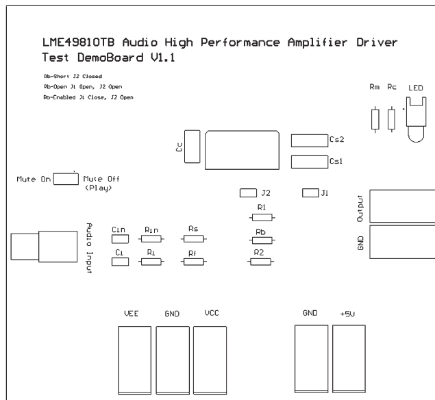
Figure 36. Silkscreen Layer
