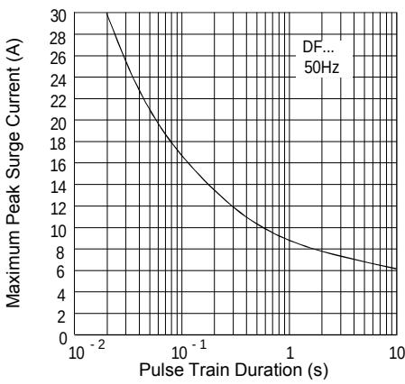
Fig. 4 - Non-Repetitive Surge Ratings
