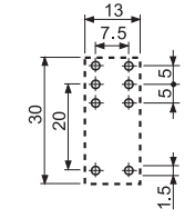
95.15.2 Copper side view
