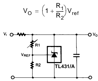
Figure 10. Shunt Regulator
